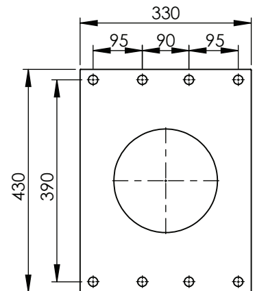
Gatenpatroon/hole pattern/ Bohrbild/motif de trous
